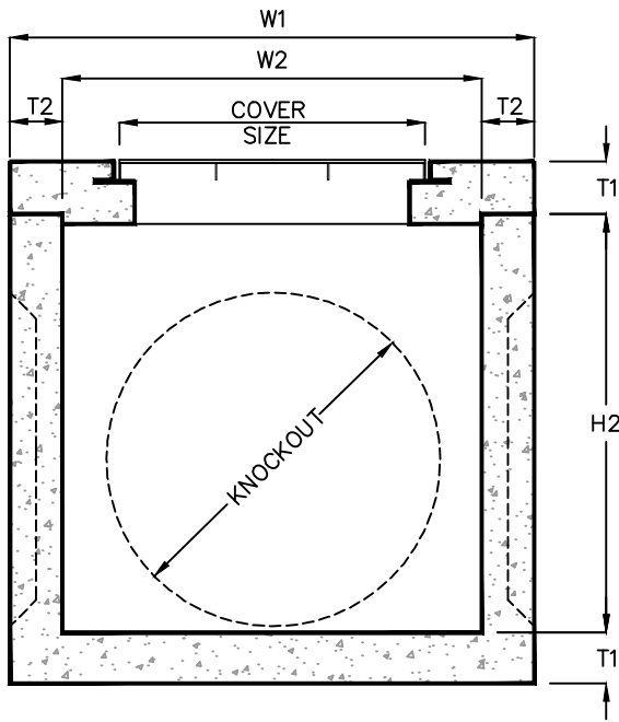
SECTION VIEW
