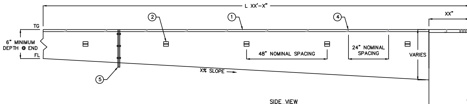
SIDE VIEW
